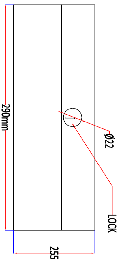
TOP VIEW
